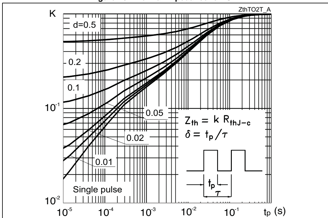
Figure 26. Thermal impedance for IGBT
