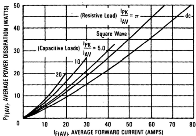
FIGURE 6 — POWER DISSIPATION
