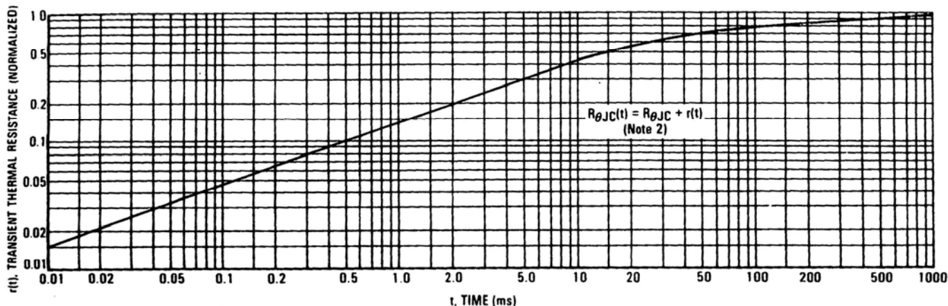
FIGURE 8 — THERMAL RESPONSE
