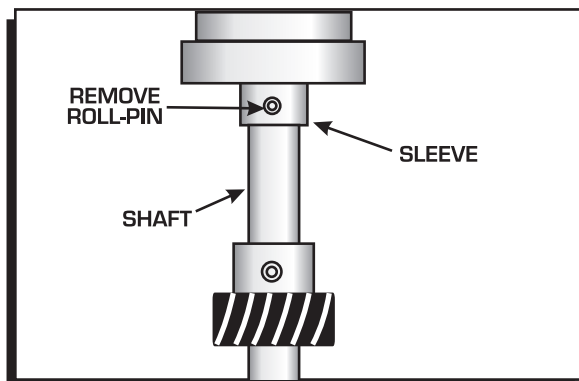
Figure 7 Removing the Retaining Sleeve.
