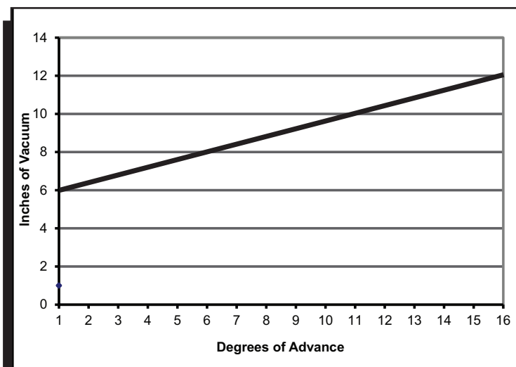
Figure 9 Vacuum Advance and Timing Chart.
