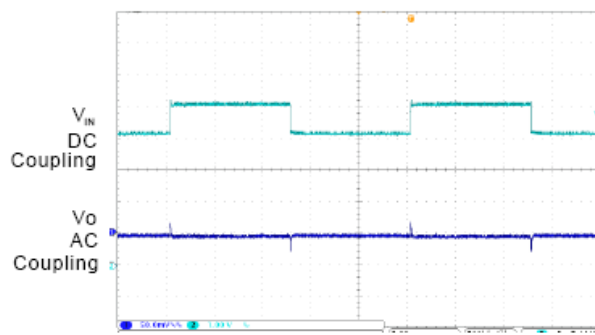
9. Line Transient
