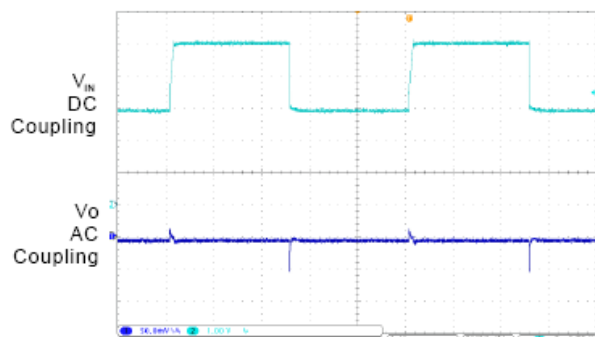
7. Line Transient
