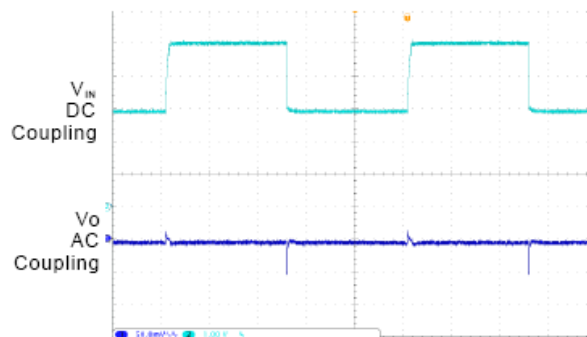
8. Line Transient
