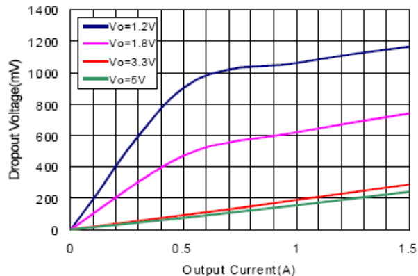
6. Dropout Voltage vs Output Current
