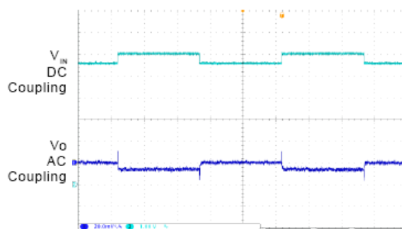
10. Line Transient
