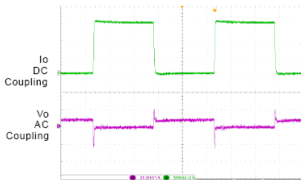
11. Load Transient
