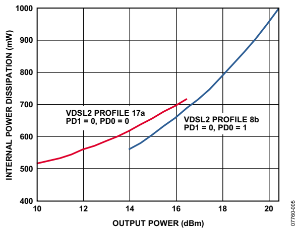
Figure 11. Internal Power Dissipation vs. Output Power
