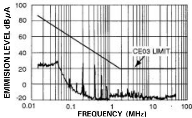
BBF2812S CONVERTER WITH BFL2805
