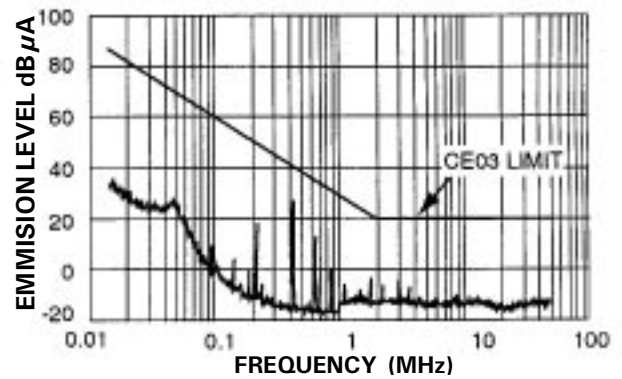
BBF2815S CONVERTER WITH BFL2805
