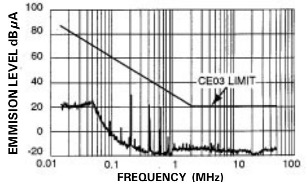
BBF2815S CONVERTER WITH BFL2805
