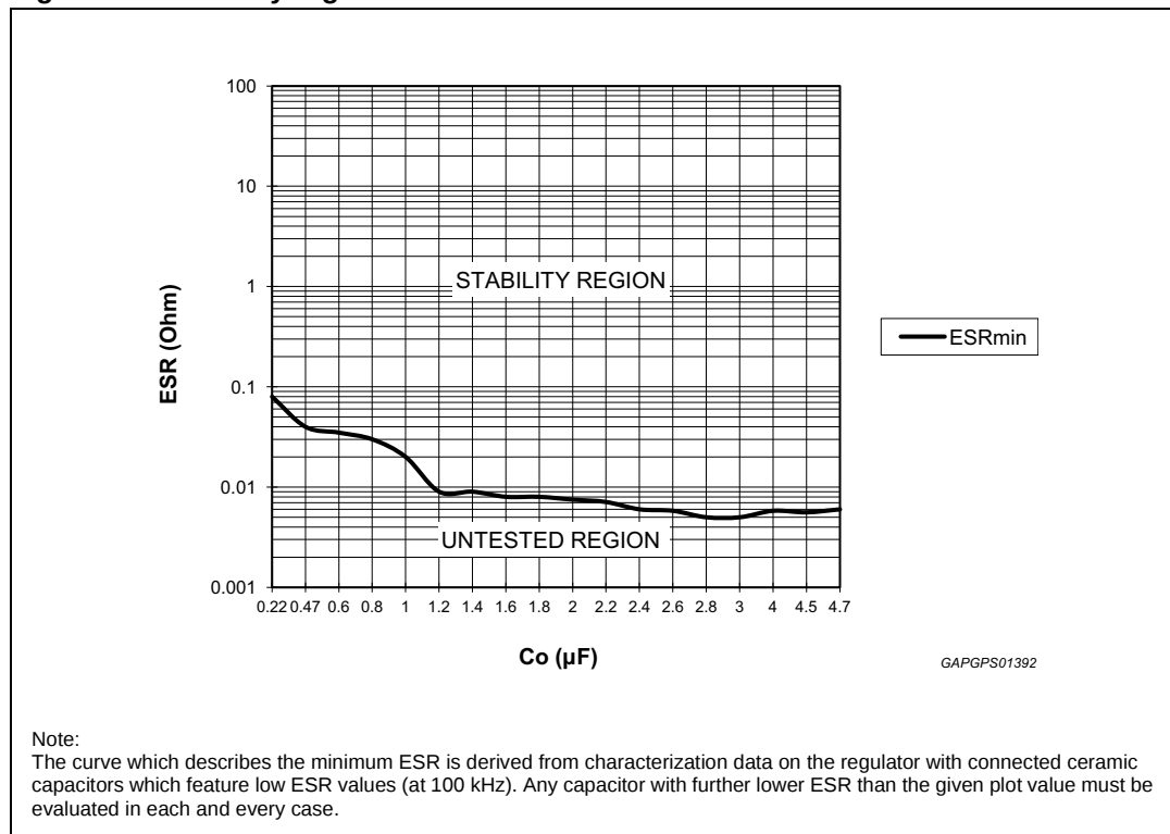
Figure 19. Stability region
