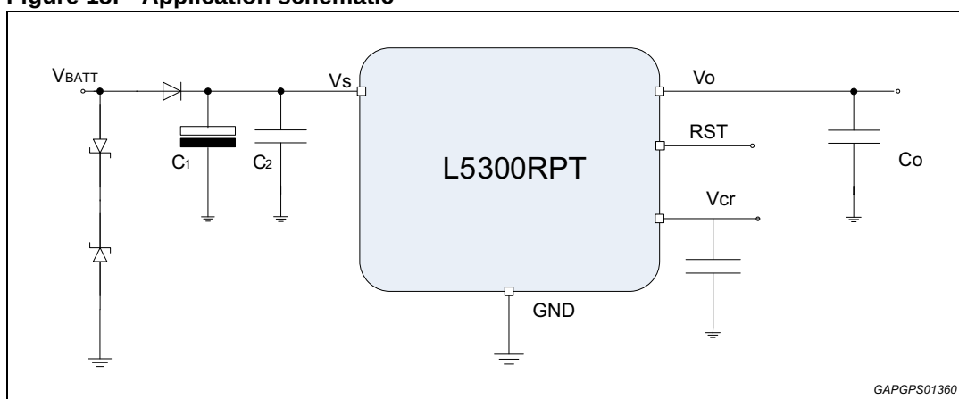
Figure 18. Application schematic
