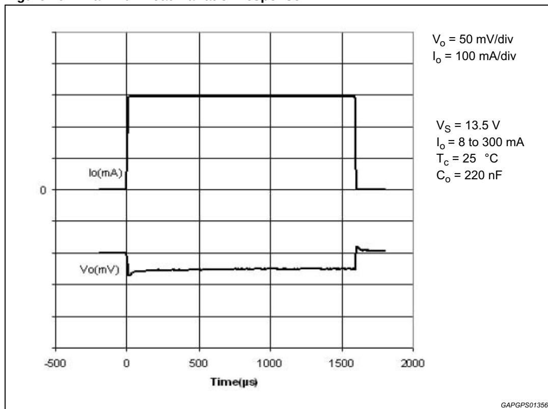
Figure 20. Maximum load variation response
