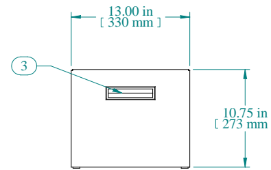
R.S. VIEW
