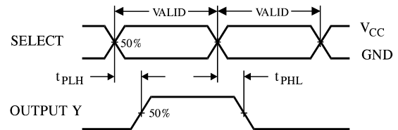
Figure 2. Switching Waveforms
