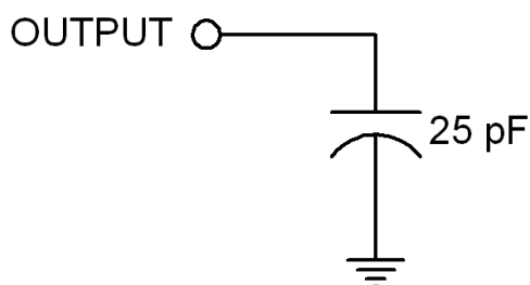
Figure 7.1 Output Equivalent Test Load
