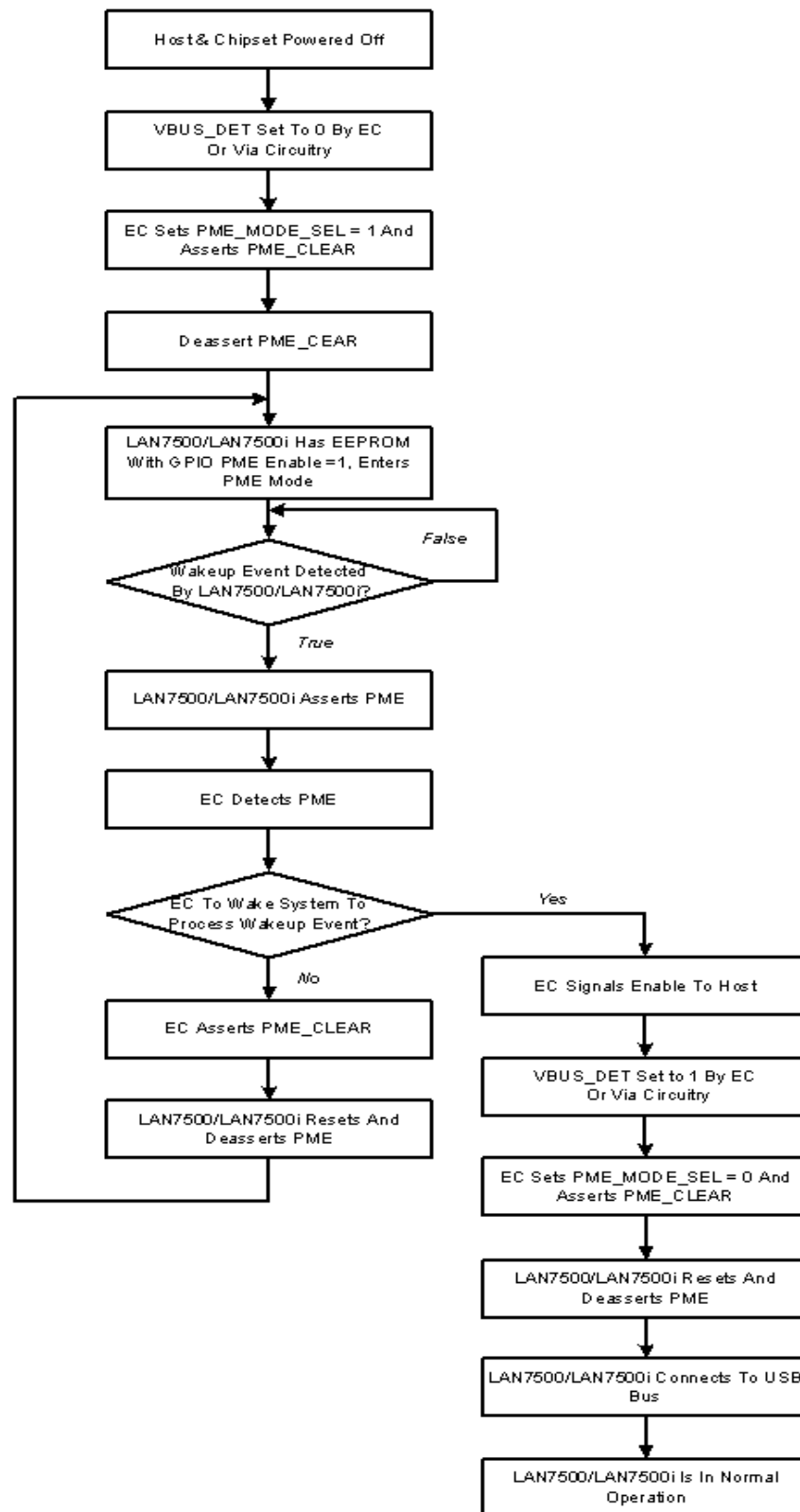
Figure 4.2 PME Operation
