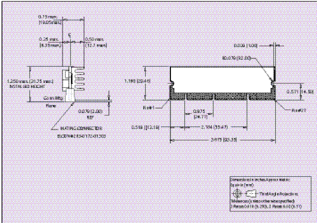
Figure 5: Mechanical Drawing
