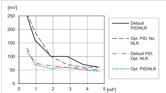
Load Transient vs. External Capacitance, V_0 = 1.0\text{ V}
