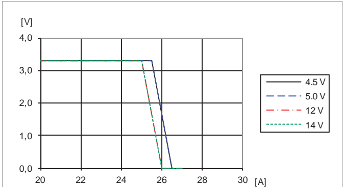
Output voltage vs. load current at T_{P1} = +25\text{ °C} , V_O = 3.3\text{ V} . Output enters hiccup mode at current limit.
