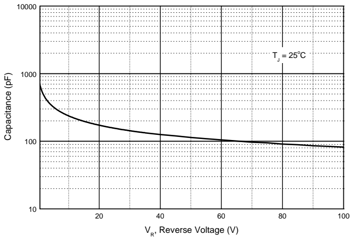
Figure 3. Capacitance vs. V_{R1} Reverse Voltage
