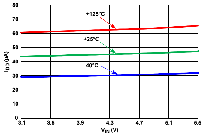
FIGURE 88. I_{IN} vs V_{IN} , OVER-TEMPERATURE
