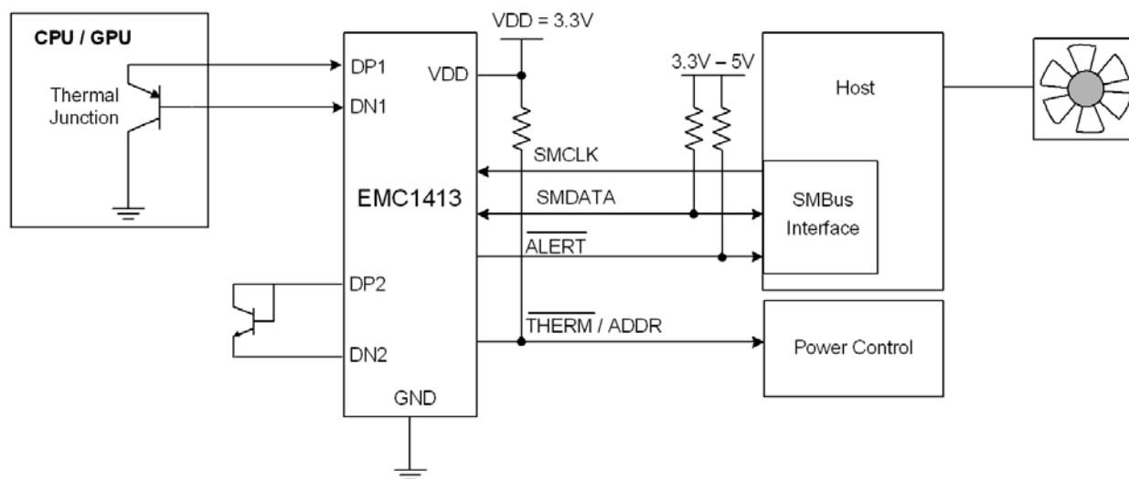
Figure 6.2 System Diagram for EMC1413
