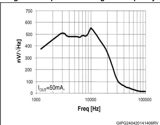
Figure 9. Output noise voltage vs. frequency
