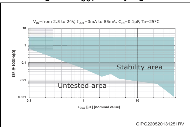
Figure 7. C_OUT stability region
