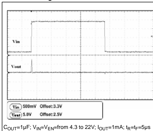
Figure 12. Line transient
