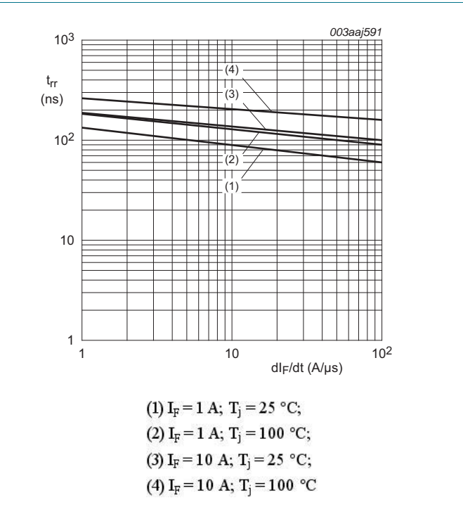
Fig 7. Reverse recovery time as a function of rate of change of forward current; maximum values
