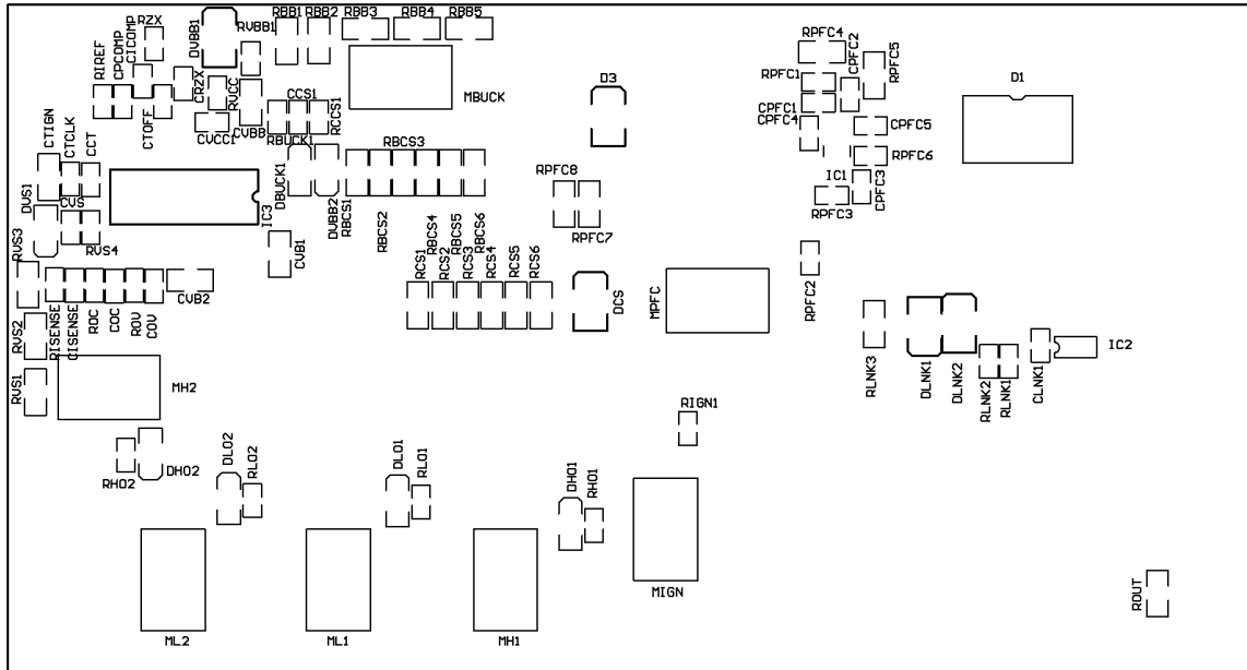
Bottom Assembly
