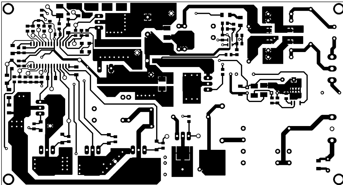
Bottom Copper
