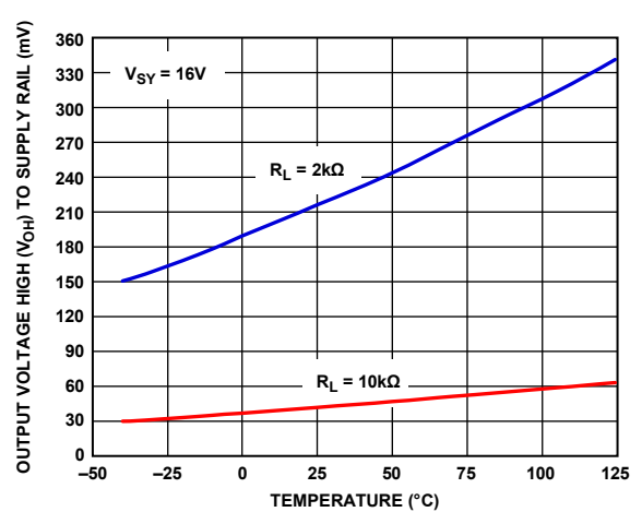
Figure 51. Output Voltage High ( V_{OH} ) to Supply Rail vs. Temperature, V_{SY} = 16V
