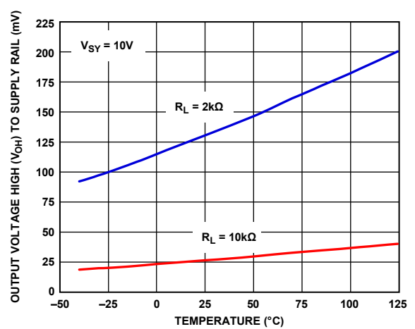
Figure 50. Output Voltage High ( V_{OH} ) to Supply Rail vs. Temperature, V_{SY} = 10V
