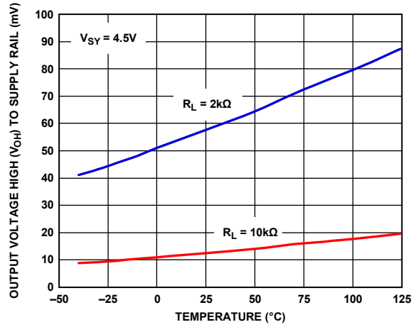
Figure 49. Output Voltage High ( V_{OH} ) to Supply Rail vs. Temperature, V_{SY} = 4.5V
