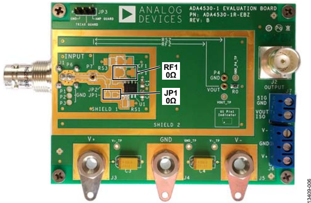
Figure 5. Buffer with Triax Guard Externally Driven
