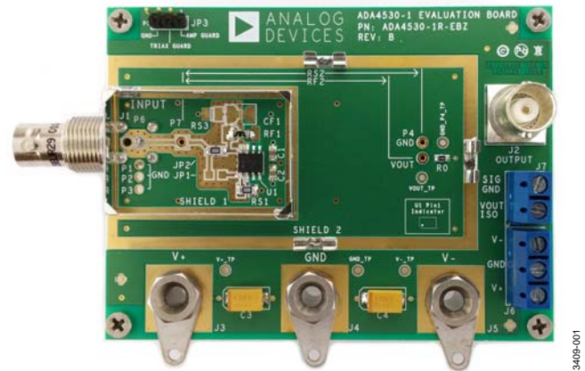
Figure 1. ADA4530-1R-EBZ Top View
