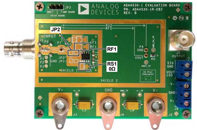
Figure 19. Inverting Gain
