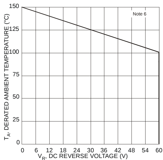
Fig. 6 Operating Temperature Derating
