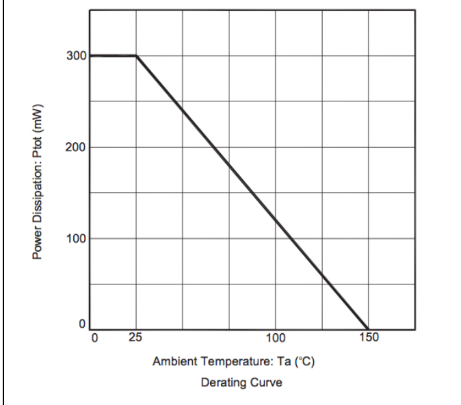
Fig 3 Power Derating
