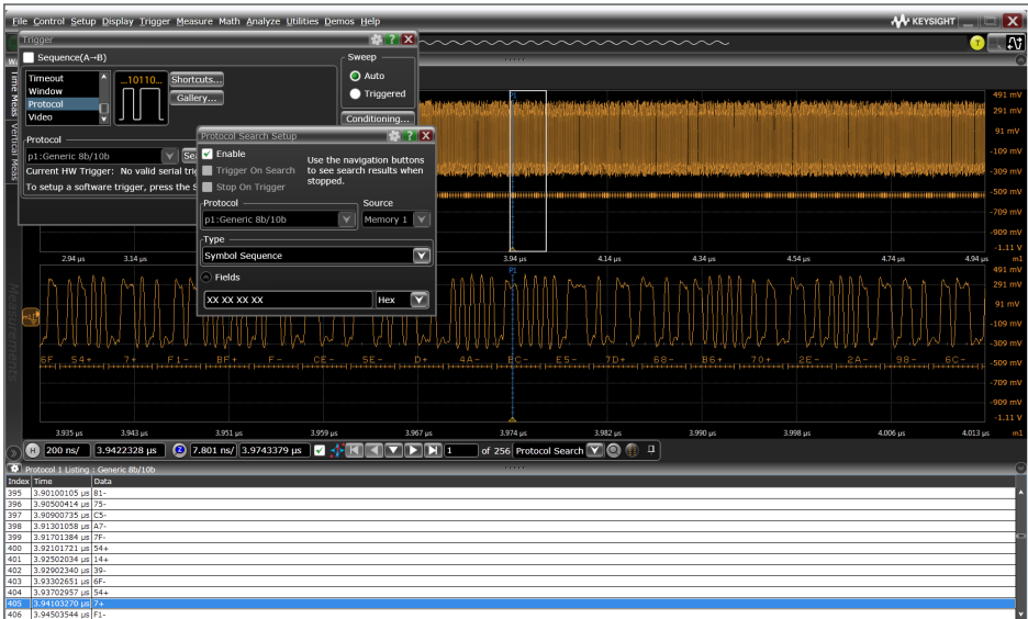
Figure 9. Configuring a serial data trigger in the 8b/10b protocol.
