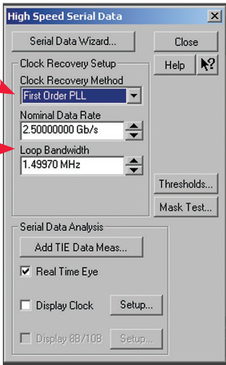
Figure 10. First-order PLL selections.
