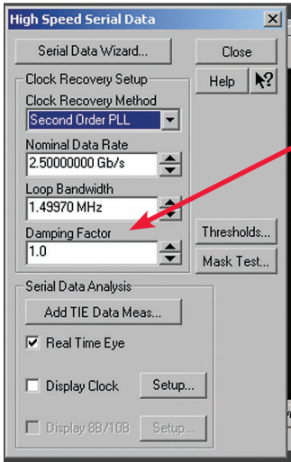
Figure 11. Second-order PLL selections.
