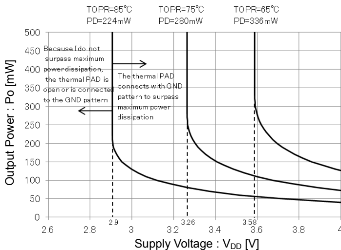
Figure 42. Handling of Thermal PAD Condition (BTL Mode)
