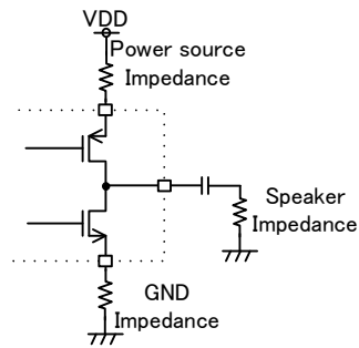
Fig. 40 Line Impedance
