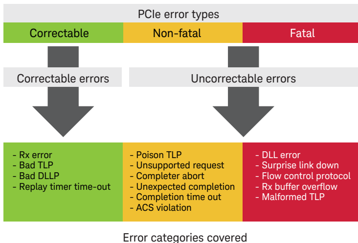
Figure 10. Using the RAS test scripts from Intel, testing fault operations provides validation of the RAS error framework.
