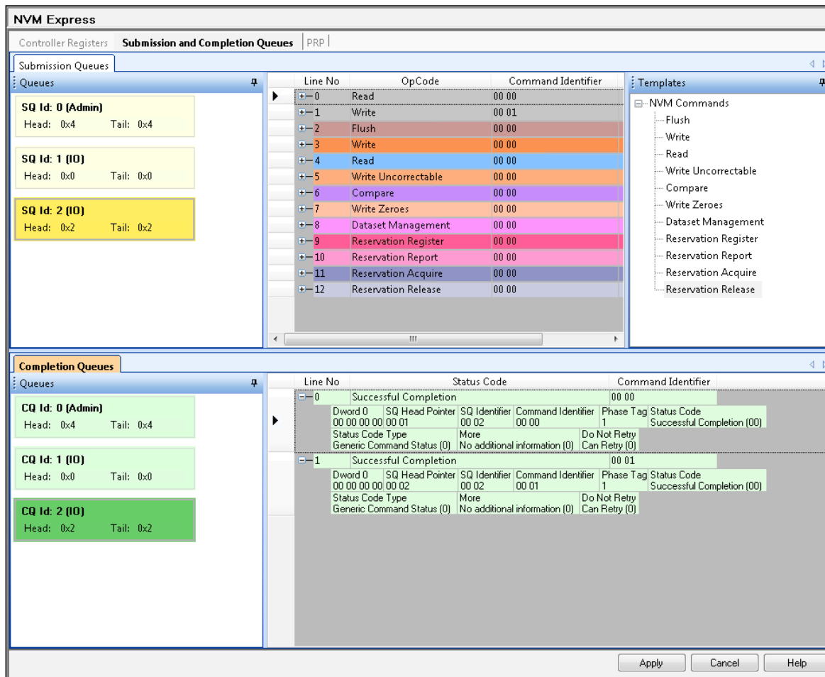
Figure 12. Create up to 64 submission and 64 completion queues, and easily execute queue management commands.
