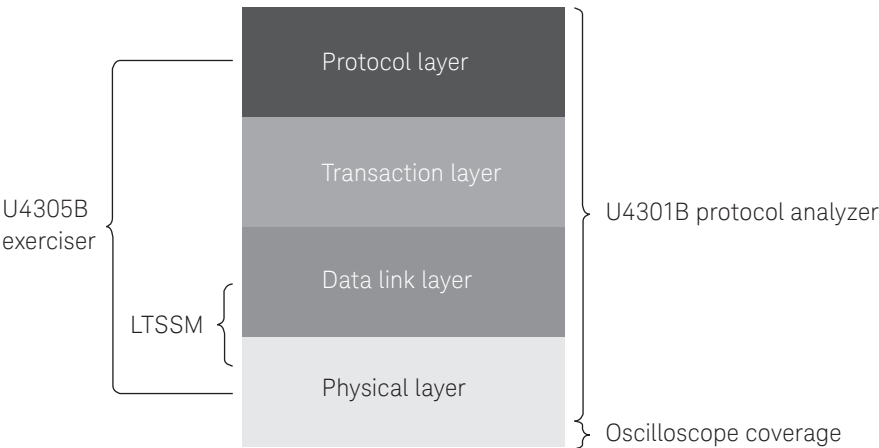
Figure 3. Application coverage of the Keysight U4305B PCIe 3.0 exerciser module.
