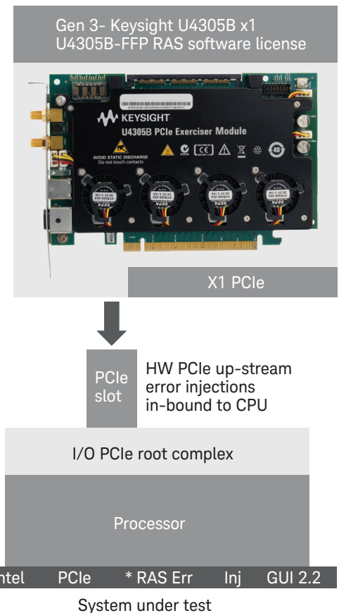
Figure 10. Using the RAS test scripts from Intel, testing fault operations provides validation of the RAS error framework.
