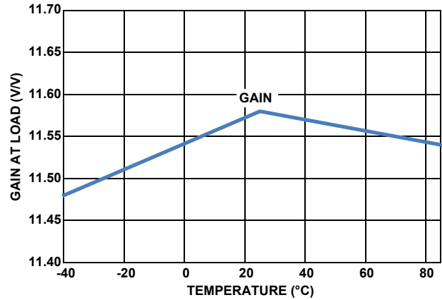
FIGURE 22. GAIN AT LOAD vs TEMPERATURE
