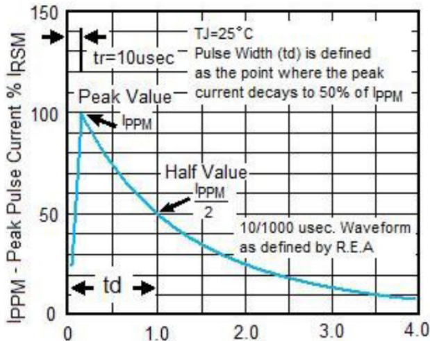
Fig.1 Pulse Waveform
