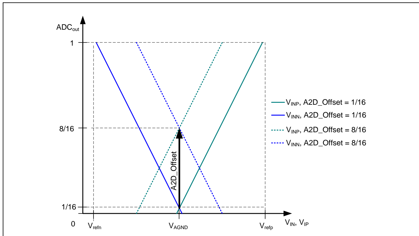
Figure 2.2 ADC Offset
