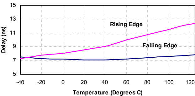
Figure 10. Propagation Delay vs. Temperature 2.5 V Operation
