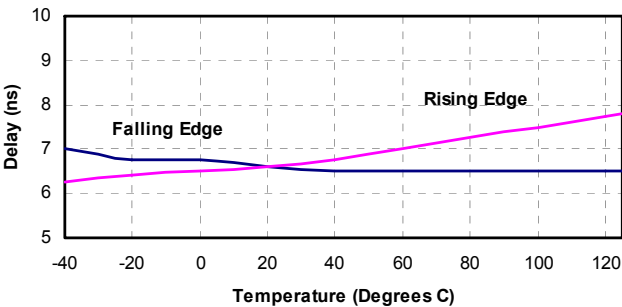
Figure 9. Propagation Delay vs. Temperature 3.3 V Operation
