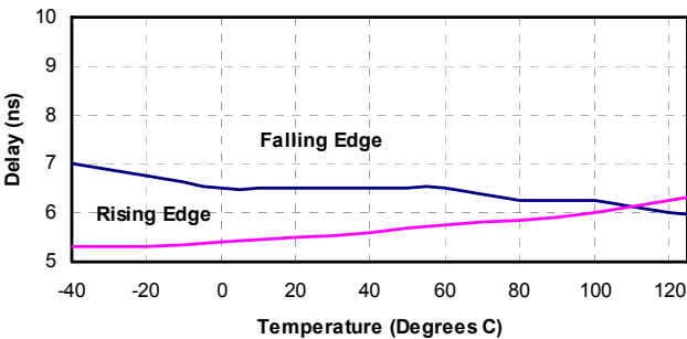
Figure 8. Propagation Delay vs. Temperature 5 V Operation
