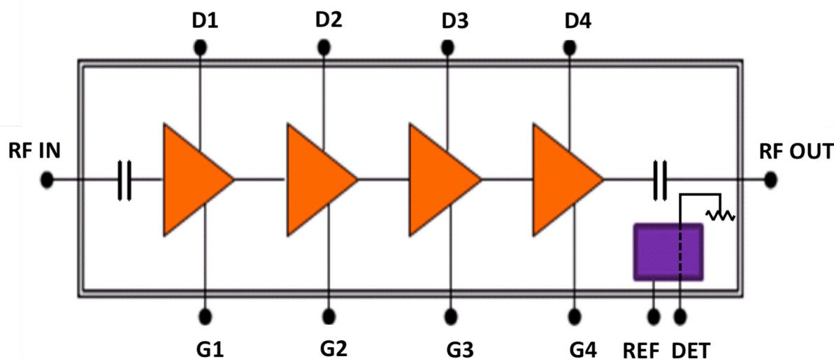
Figure 1: Device diagram
