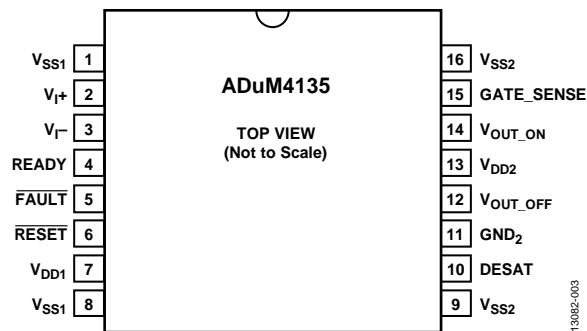
Figure 3. Pin Configuration
