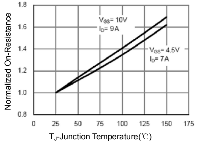
Figure 8 Drain-Source On-Resistance
