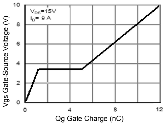
Figure 11 Gate Charge
