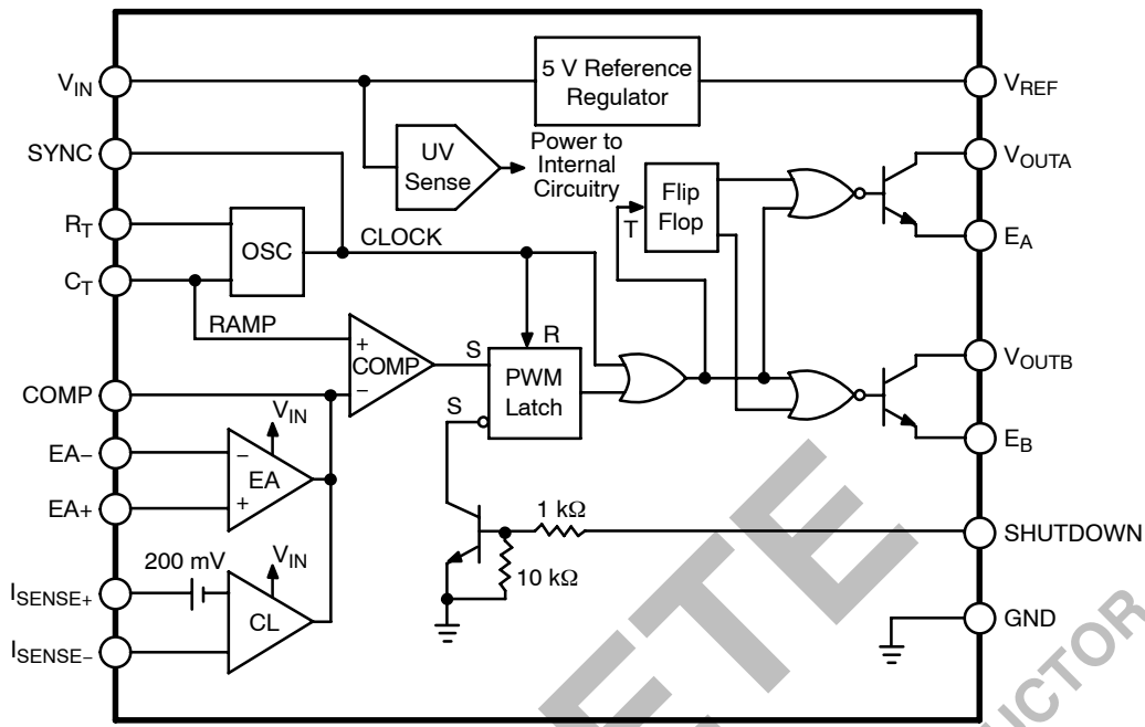
Figure 1. Block Diagram
