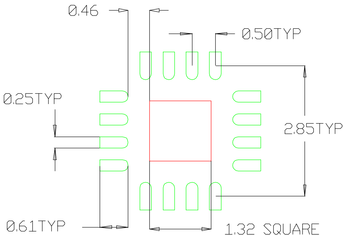
Stencil Aperture All Dimensions in mm
