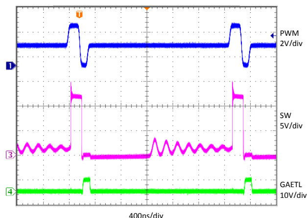
Figure 6: Body-Braking® Mode
