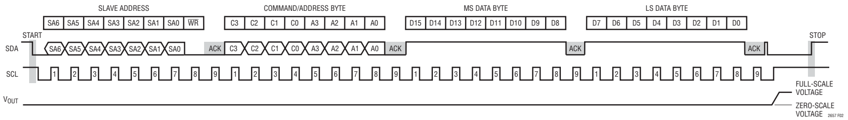
Figure 2. Typical LTC2657 Input Waveform –Programming DAC Output for Full-Scale
