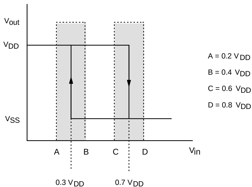
Figure 13-3. Schmitt Trigger Input Characteristics Diagram
