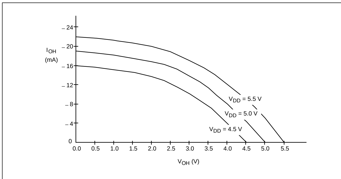
Figure 13-9. I_{OH} vs. V_{OH} (P1-P3, T_A = 25\text{ }^{\circ}\text{C} )
