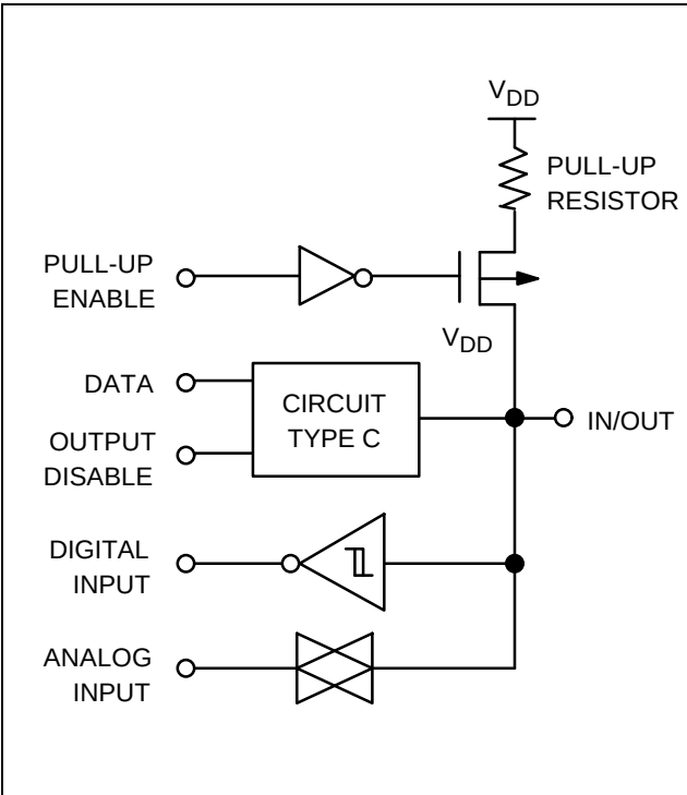
Figure 1-12. Pin Circuit Type F
