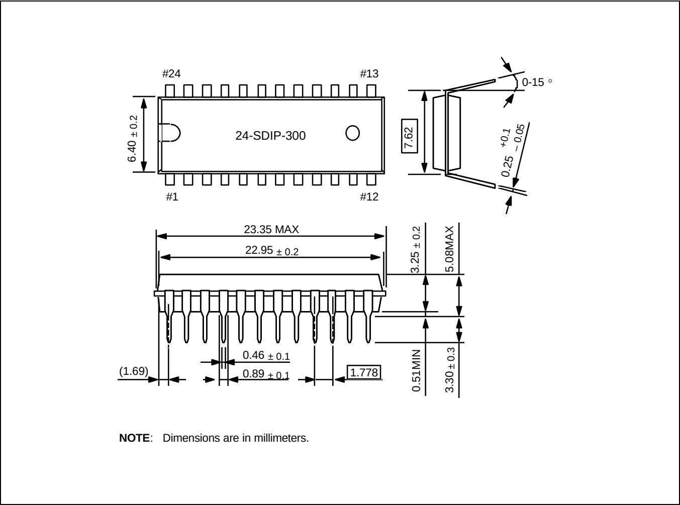
Figure 14-3. 24-SDIP-300 Package Dimensions
