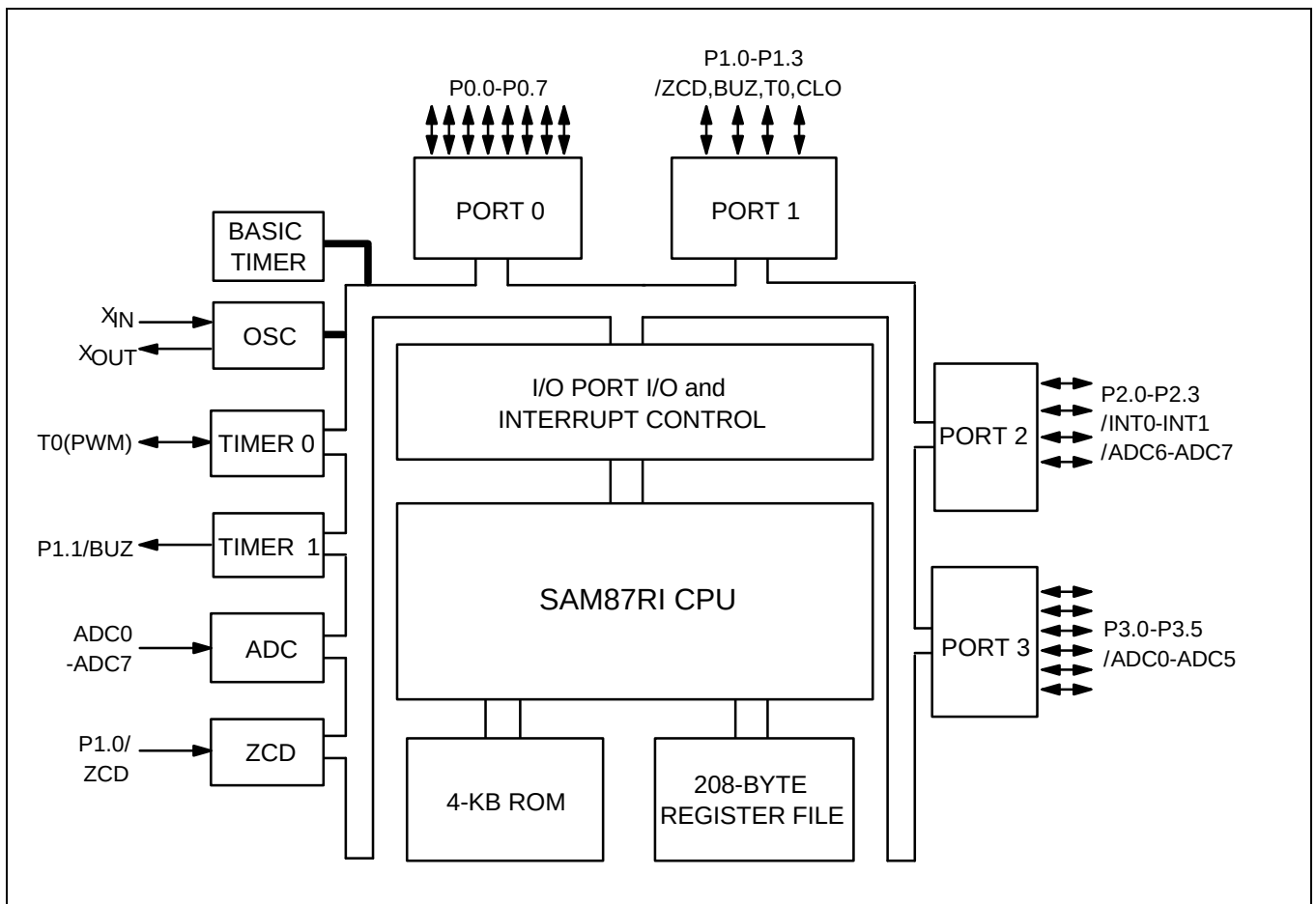
Figure 1-1. Block Diagram
