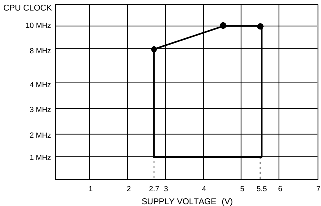
Figure 13-2. Operating Voltage Range
