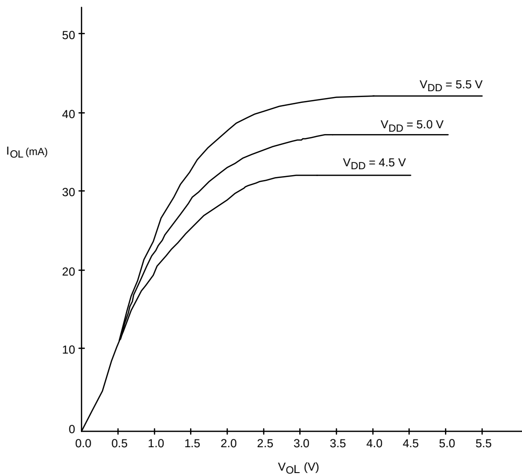
Figure 13-7. I_{OL} vs. V_{OL} (P1-P3, T_A = 25^\circ\text{C} )
