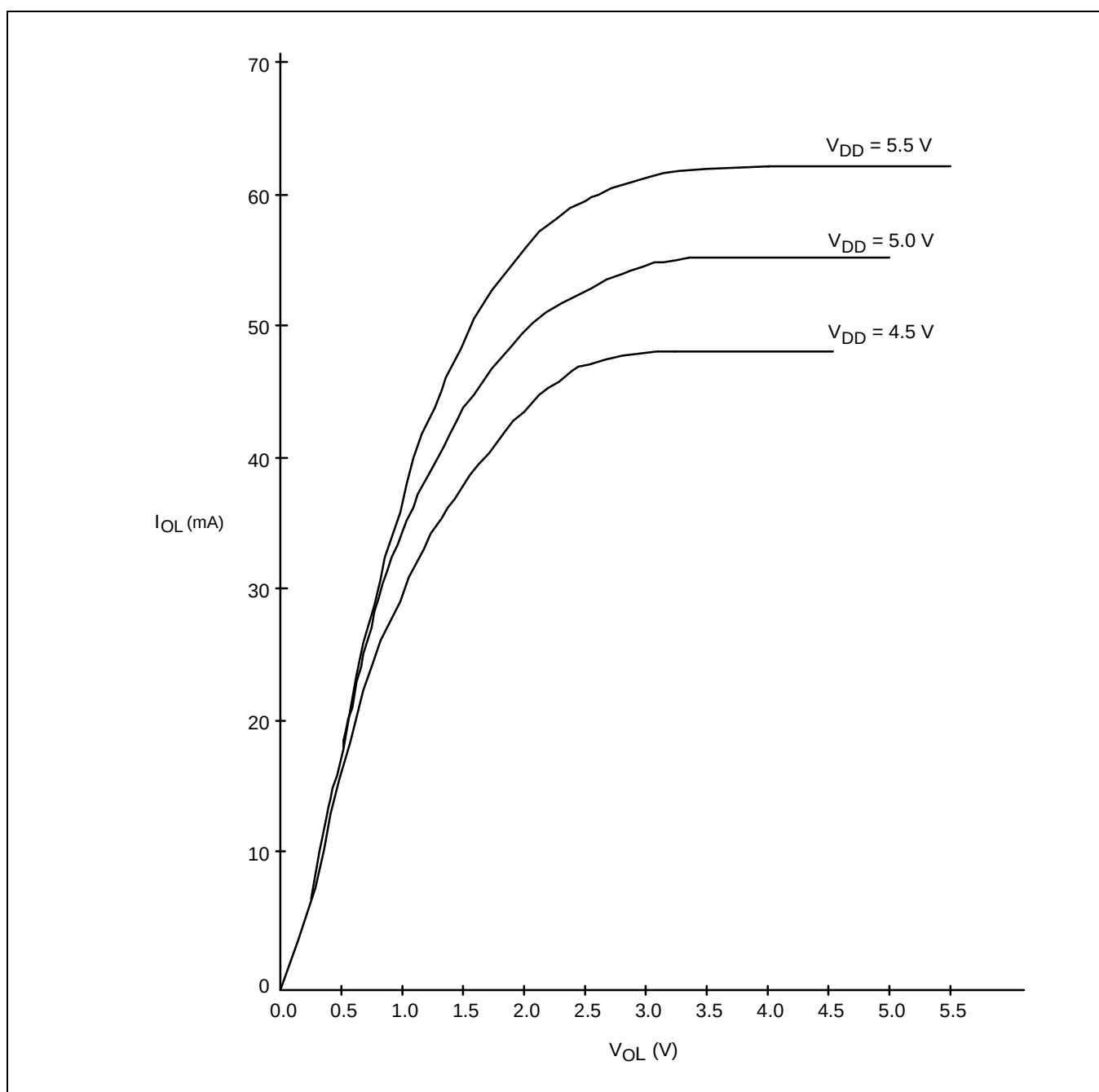
Figure 13-6. I_{OL} vs. V_{OL} (P0, T_A = 25\text{ }^{\circ}\text{C} )
