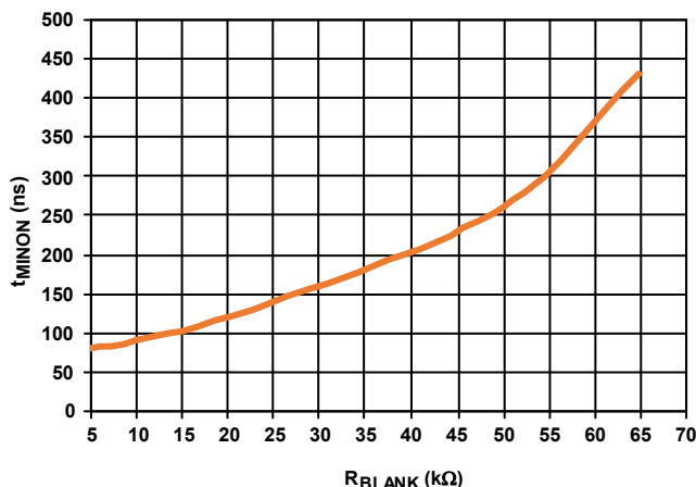
FIGURE 66. t_{\text{MINON}} vs R_{\text{BLANK}}
