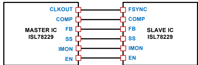
FIGURE 63. CONFIGURATIONS FOR DUAL IC 4-PHASE OPERATION
