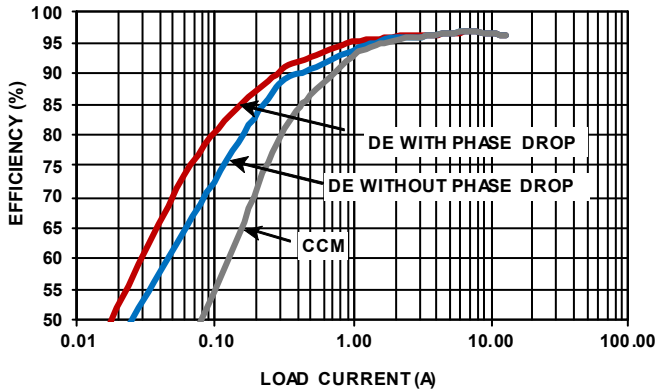
NOTE: (See Typical Application in Figure 4 on page 8 .) FIGURE 5. EFFICIENCY vs LOAD, 2-PHASE BOOST, 3 MODES OPERATION, f_{SW} = 200kHz , V_{IN} = 12V , V_{OUT} = 36V , T_A = +25^\circ C
