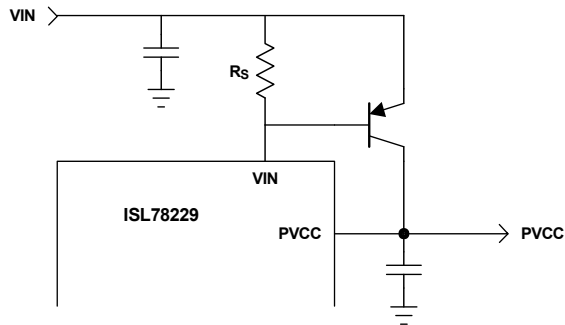
FIGURE 73. SUPPLEMENTING LDO CURRENT
