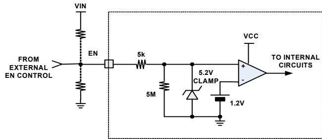
FIGURE 68. ENABLE BLOCK
