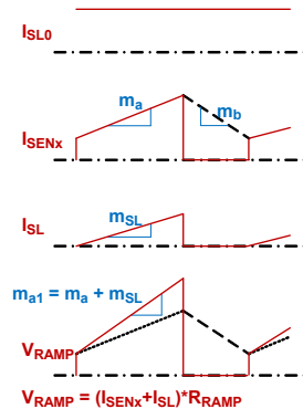
FIGURE 70. SLOPE COMPENSATION BLOCK DIAGRAM
