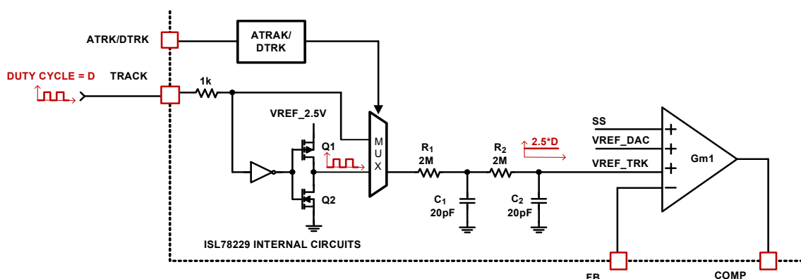
FIGURE 60. TRACK FUNCTION BLOCK DIAGRAM
