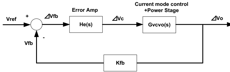
FIGURE 75. CONCEPTUAL CONTROL BLOCK DIAGRAM
