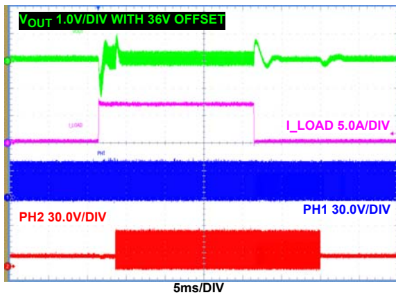
FIGURE 33. DE+PH_DROP MODE (DE/PHDRP = FLOAT), TRANSIENT RESPONSE, I_{OUT} = 1 TO 8A STEP LOAD
