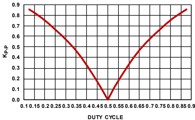
FIGURE 62. K_{P,P} vs DUTY CYCLE
