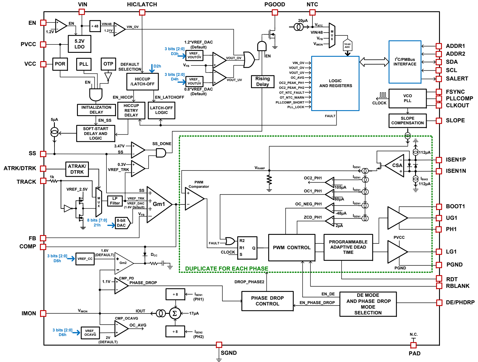
FIGURE 3. BLOCK DIAGRAM
