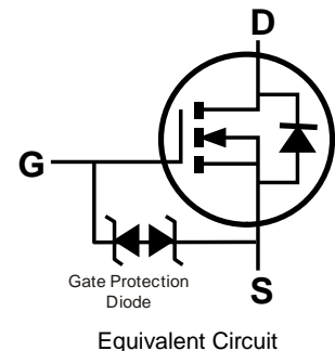
Equivalent Circuit
