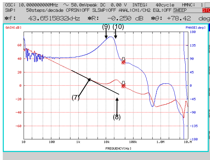
Figure 36. Example of DC/DC Converter Frequency Property (Measured with FRA5097 by NF Corporation)
