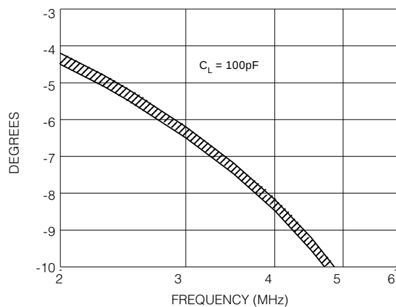
Fig. 7 GB4550A Phase Delay Spread
