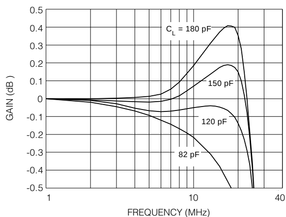
Fig. 4 GB4550 Frequency Response
