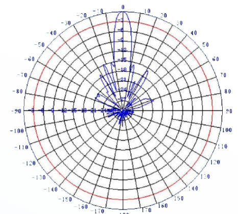
E Plane 4940 MHz
