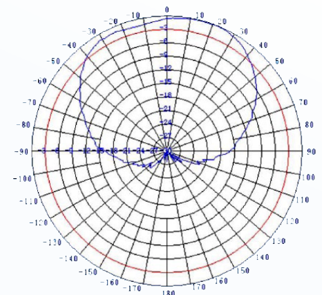
H Plane 4940 MHz
