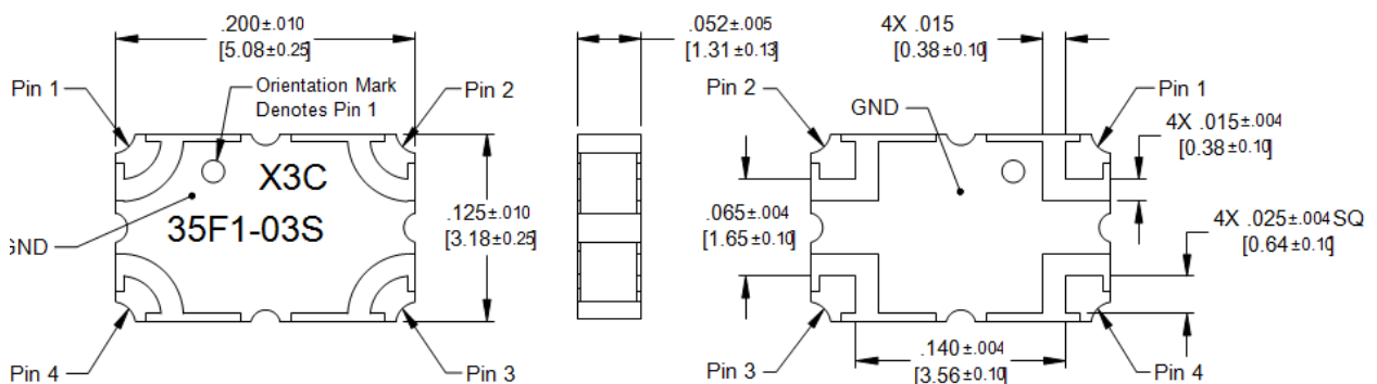
Dimensions are in Inches [Millimeters] X3C35F1-03S Mechanical Outline
