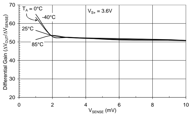
Differential Gain vs. Sense Voltage
