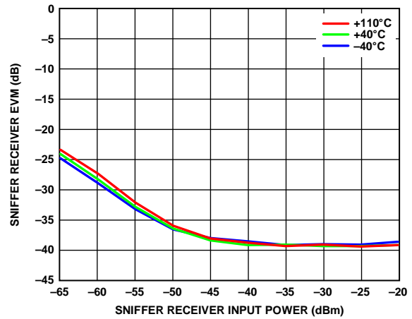
Figure 238. Sniffer Receiver EVM vs. Sniffer Receiver Input Power, 5600 MHz LO, 20 MHz RF BW, LTE 20 MHz Uplink Centered at DC, BTC Active, 30.72 MSPS Sample Rate
