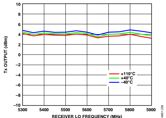
Figure 199. Tx Output Power, Transmitter QEC, and External LO Leakage Active, 5 MHz CW Offset Signal, 1 MHz Resolution Bandwidth, 245.76 MSPS Sample Rate
