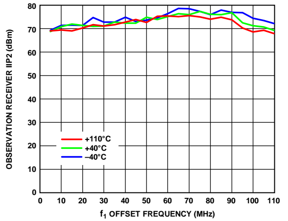
Figure 45. Observation Receiver IIP2 vs. f_1 Offset Frequency, 900 MHz LO, 0 dB Attenuation, 100 MHz RF Bandwidth, f_2 = f_1 + 1 MHz, 122.88 MSPS Sample Rate
