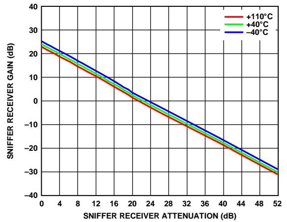
Figure 239. Sniffer Receiver Gain vs. Sniffer Receiver Attenuation, 5800 MHz LO, CW Signal 3 MHz Offset, 20 MHz RF BW, 30.72 MSPS Sample Rate
