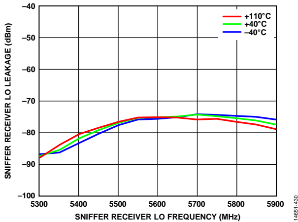
Figure 230. Sniffer Receiver LO Leakage vs. Sniffer Receiver LO Frequency, 0 dB Receiver Attenuation, 20 MHz RF BW, 30.72 MSPS Sample Rate
