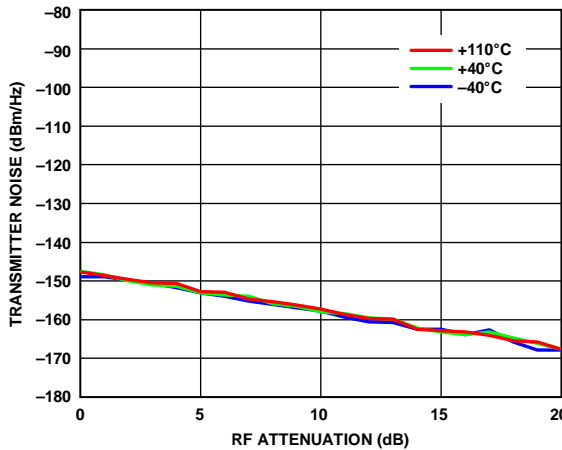
Figure 29. Transmitter Noise vs. RF Attenuation, 800 MHz LO, 20 MHz Offset Frequency
