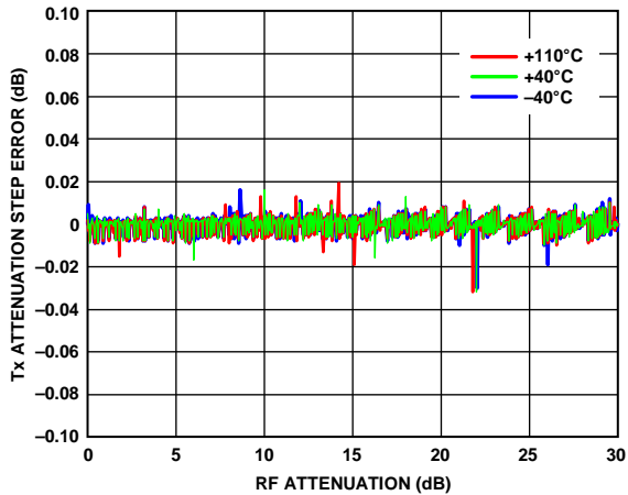
Figure 41. Tx Attenuation Step Error vs. RF Attenuation, 800 MHz LO, 810 MHz CW Desired Signal, 20 MHz RF Bandwidth, 122.88 MSPS Sample Rate
