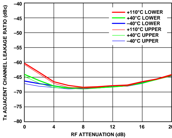
Figure 30. Tx Adjacent Channel Leakage Ratio vs. RF Attenuation, 900 MHz LO, 20 MHz RF Bandwidth, Four-Carrier W-CDMA Desired Signal, Transmitter QEC and LO Leakage Tracking Active
