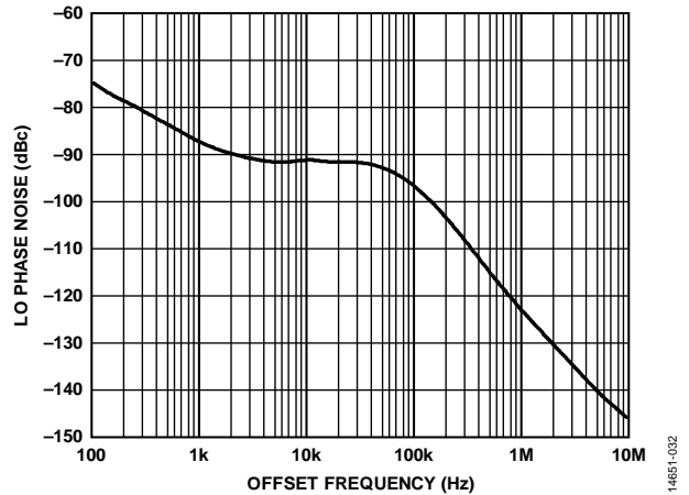
Figure 91. LO Phase Noise vs. Offset Frequency, 3 dB Digital Backoff, 2600 MHz
