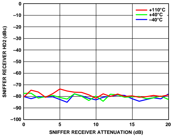
Figure 236. Sniffer Receiver HD2 vs. Sniffer Receiver Attenuation, 5800 MHz LO, CW Signal 3 MHz Offset, -35 dBm at 0 dB Attenuation, Input Power Increasing dB for dB with Attenuation, 20 MHz RF BW, 30.72 MSPS Sample Rate
