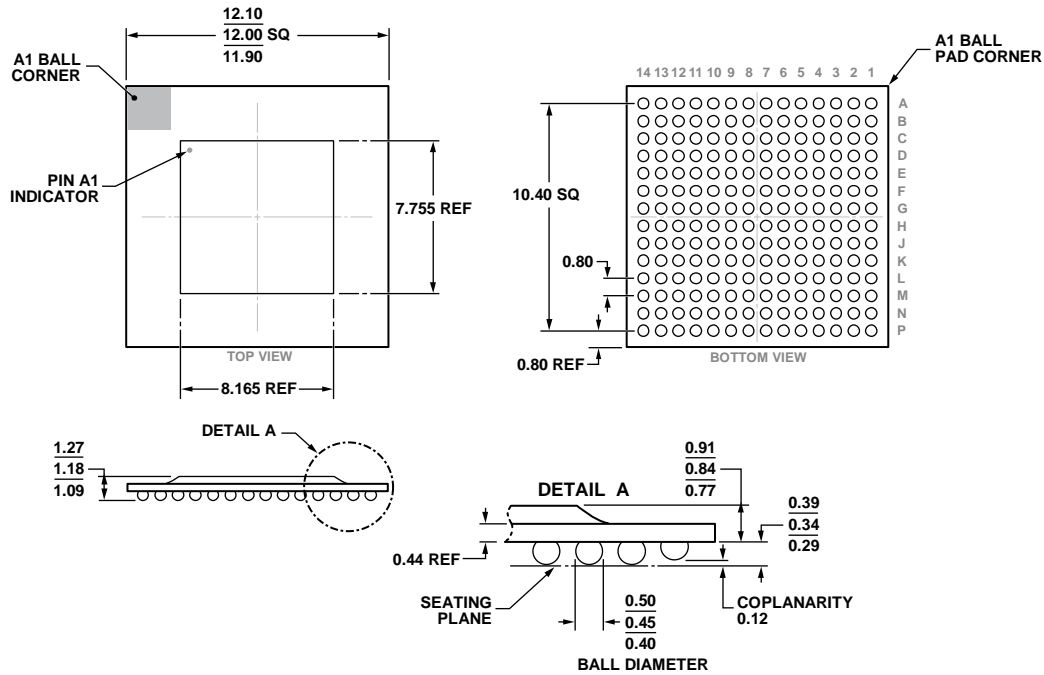
COMPLIANT TO JEDEC STANDARDS MO-275-GGAB-1. Figure 242. 196-Ball Chip Scale Package Ball Grid Array [CSP_BGA] (BC-196-12) Dimensions shown in millimeters
