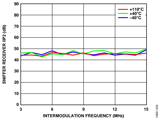
Figure 232. Sniffer Receiver IIP2 vs. Intermodulation Frequency ( f_2 - f_1 ), 5600 MHz LO, 0 dB Attenuation, 20 MHz RF BW, 30.72 MSPS Sample Rate
