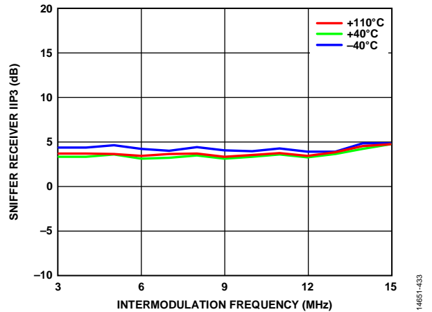
Figure 233. Sniffer Receiver IIP3 vs. Intermodulation Frequency ( f_2 - 2f_1 ), 5600 MHz LO, 0 dB Attenuation, 20 MHz RF BW, 30.72 MSPS Sample Rate
