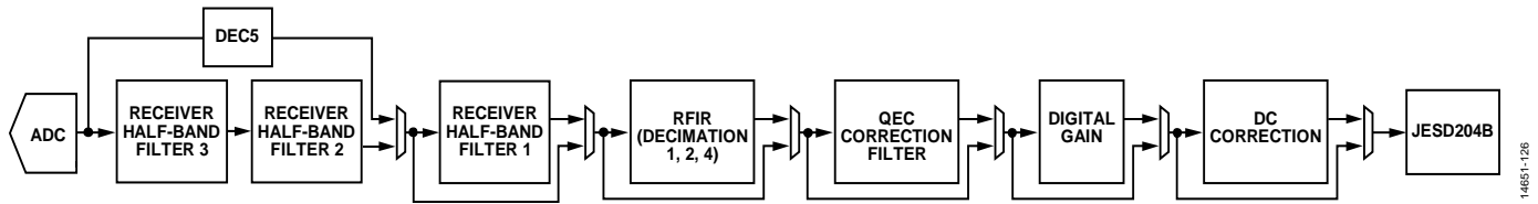
Figure 241. Data Rx Data Path Filter Implementation
