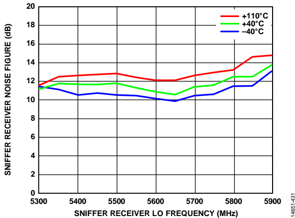
Figure 231. Sniffer Receiver Noise Figure vs. Sniffer Receiver LO Frequency, 0 dB Receiver Attenuation, 20 MHz RF BW, 38.4 MSPS Sample Rate, 10 MHz Integration BW
