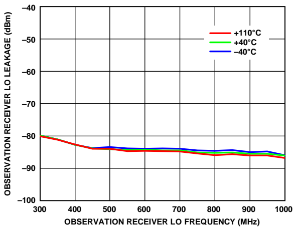
Figure 43. Observation Receiver LO Leakage vs. Observation Receiver LO Frequency, 0 dB Receiver Attenuation, 100 MHz RF Bandwidth, 122.88 MSPS Sample Rate
