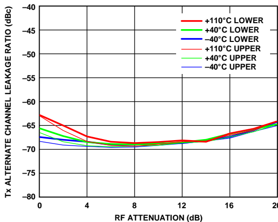
Figure 31. Tx Alternate Channel Leakage Ratio vs. RF Attenuation, 900 MHz LO, 20 MHz RF Bandwidth, Four-Carrier W-CDMA Desired Signal, 2 dB Digital Backoff, Transmitter QEC and LO Leakage Tracking Active
