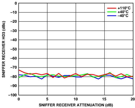
Figure 237. Sniffer Receiver HD3 vs. Sniffer Receiver Attenuation, 5800 MHz LO, CW Signal 3 MHz Offset, -35 dBm at 0 dB Attenuation, Input Power Increasing dB for dB with Attenuation, 20 MHz RF BW, 30.72 MSPS Sample Rate
