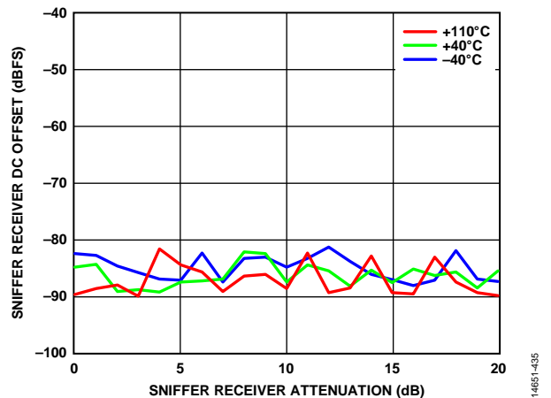
Figure 235. Sniffer Receiver DC Offset vs. Sniffer Receiver Attenuation, 5800 MHz LO, CW Signal 3 MHz Offset, -35 dBm at 0 dB Attenuation, Input Power Increasing dB for dB with Attenuation, 20 MHz RF BW, 30.72 MSPS Sample Rate
