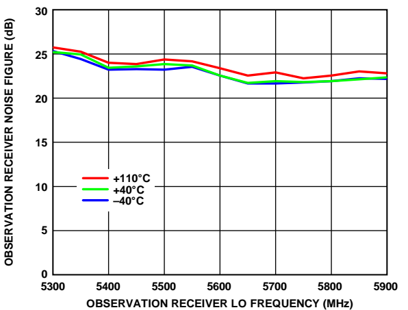
Figure 220. Observation Receiver Noise Figure vs. Observation Receiver LO Frequency, 0 dB Receiver Attenuation, 200 MHz RF Bandwidth, 245.76 MSPS Sample Rate, 100 MHz Integration Bandwidth
