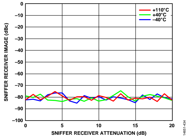
Figure 234. Sniffer Receiver Image vs. Sniffer Receiver Attenuation, 5800 MHz LO, CW Signal 3 MHz Offset, 20 MHz RF BW, 30.72 MSPS Sample Rate
