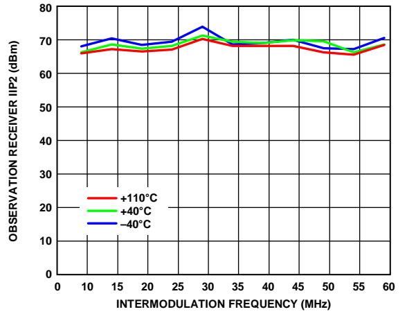
Figure 46. Observation Receiver IIP2 vs. Intermodulation Frequency ( f_2 - f_1 ), 900 MHz LO, 0 dB Attenuation, 100 MHz RF Bandwidth, 122.88 MSPS Sample Rate
