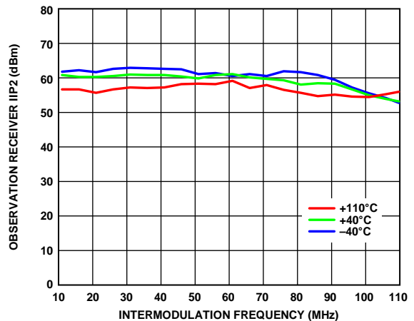
Figure 222. Observation Receiver IIP2 vs. Intermodulation Frequency ( f_2 - f_1 ), 5600 MHz LO, 0 dB Attenuation, 200 MHz RF Bandwidth, 245.76 MSPS Sample Rate
