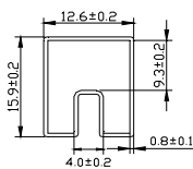
TUBE MECHANICAL DIMENSION
