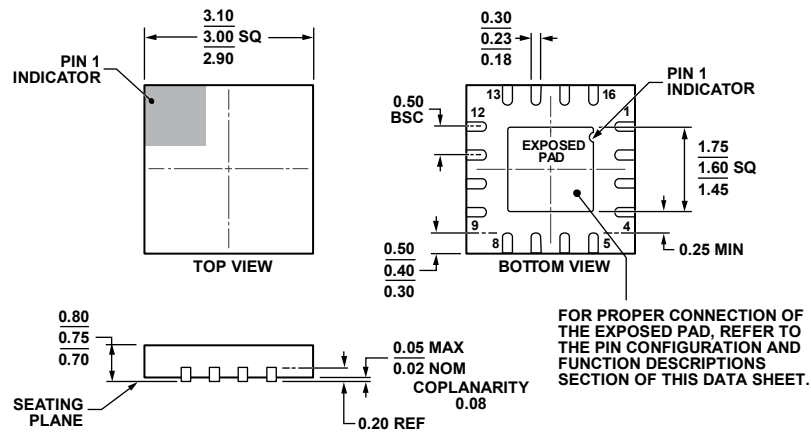
Figure 47. 16-Lead Lead Frame Chip Scale Package [LFCSP] 3 mm × 3 mm Body and 0.75 mm Package Height (CP-16-22)
