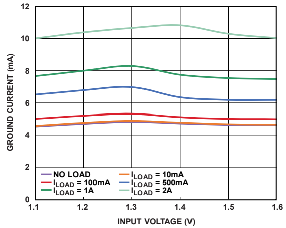
Figure 13. Ground Current vs. Input Voltage (in Dropout), V_{OUT} = 1.3 V
