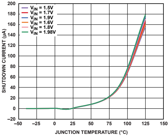
Figure 10. Shutdown Current vs. Junction Temperature at Various Input Voltages ( V_{IN} )
