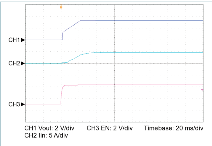
Figure 14 — Startup from EN, V_{IN} = 28\text{ V} , C_{OUT\_EXT} = 20000\ \mu\text{F} , R_{LOAD} = 0.091\ \Omega
