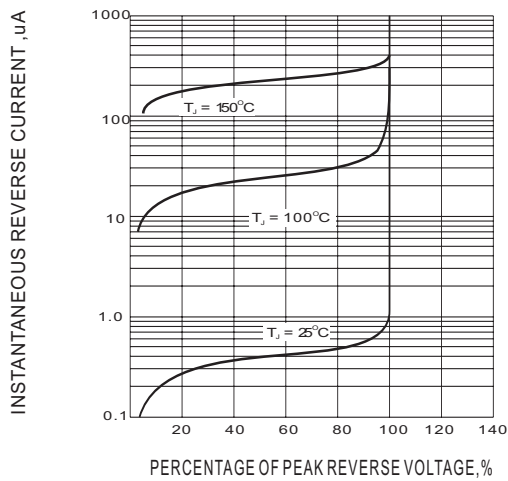
Fig. 3-TYPICAL REVERSE CHARACTERISTIC
