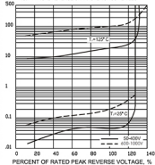
FIG.4-TYPICAL REVERSE CHARACTERISTICS PER LEG
