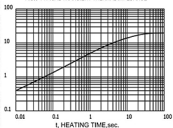
FIG.6-TYPICAL TRANSIENT THERMAL IMPEDANCE
