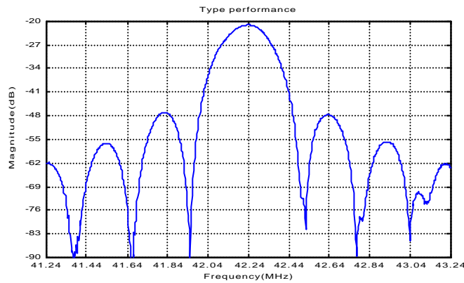
LBS42.24 SAW Filter Typical Performance
